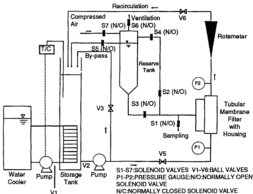
FIG. 1 Experimental setup of CFMF with periodic backflush cleaning technique.
