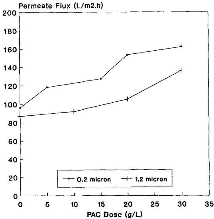
FIG. 5 Comparison of permeate flux at different doses of PAC using 0.2 and 1.2- \mu m membranes.
